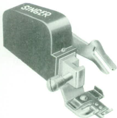
FIG. 83. THE BLIND STITCHER.
