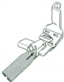
FIG. 71. INSERTING BINDING IN BINDER.
