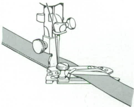
FIG. 92. HEMMING WITH THE ADJUSTABLE HEMMER.
