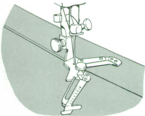
FIG. 94. HEMMER ADJUSTED FOR WIDE HEMMING.
