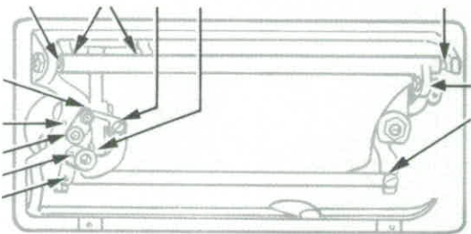
FIG. 51. OILING POINTS BELOW BED OF MACHINE 66K.
