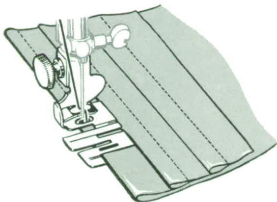
FIG. 130. TUCKING WITH THE EDGE-STITCHER.
