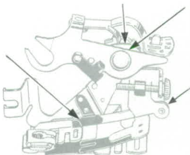
FIG. 100. OILING POINTS ON RUFFLER.
