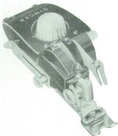
FIG. 141. ZIGZAGGER FOR 15K AND 201K MACHINES.
