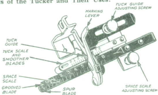
FIG. 95. THE TUCKER AND ITS WORKING PARTS.
