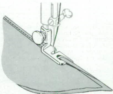
FIG. 89. MAKING A HEMMED SEAM.
