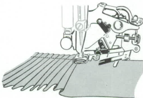
FIG. 105. THE RUFFLER ADJUSTED FOR PLAITING.
