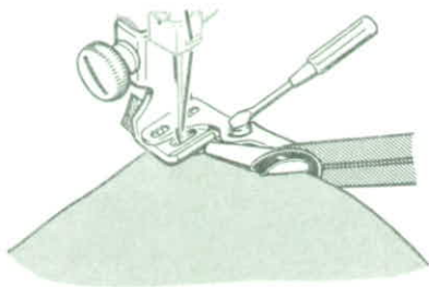
FIG. 73. ADJUSTING THE BINDER.
