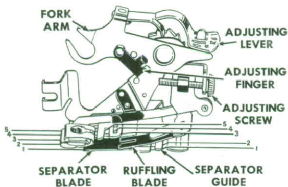
FIG. 99. THE RUFFLER AND ITS PARTS.
