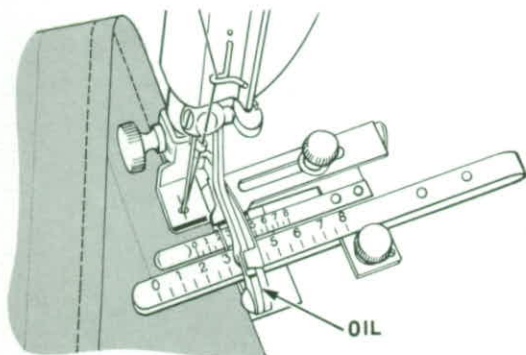
FIG. 97. PROPER POSITION OF MATERIAL IN TUCKER.
