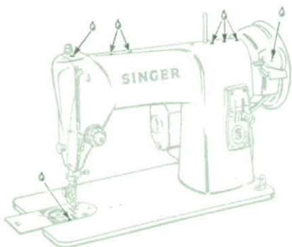
FIG. 48a. CLEANING AND OILING THE HEAD.
