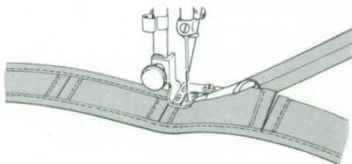
FIG. 81. COMPLETING BOUND BUTTONHOLES.
