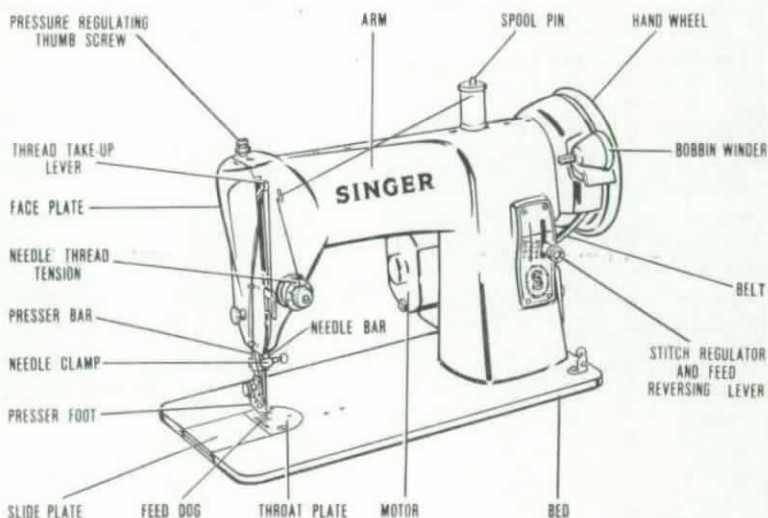
FIG. 1. PRINCIPAL PARTS OF THE HEAD.
